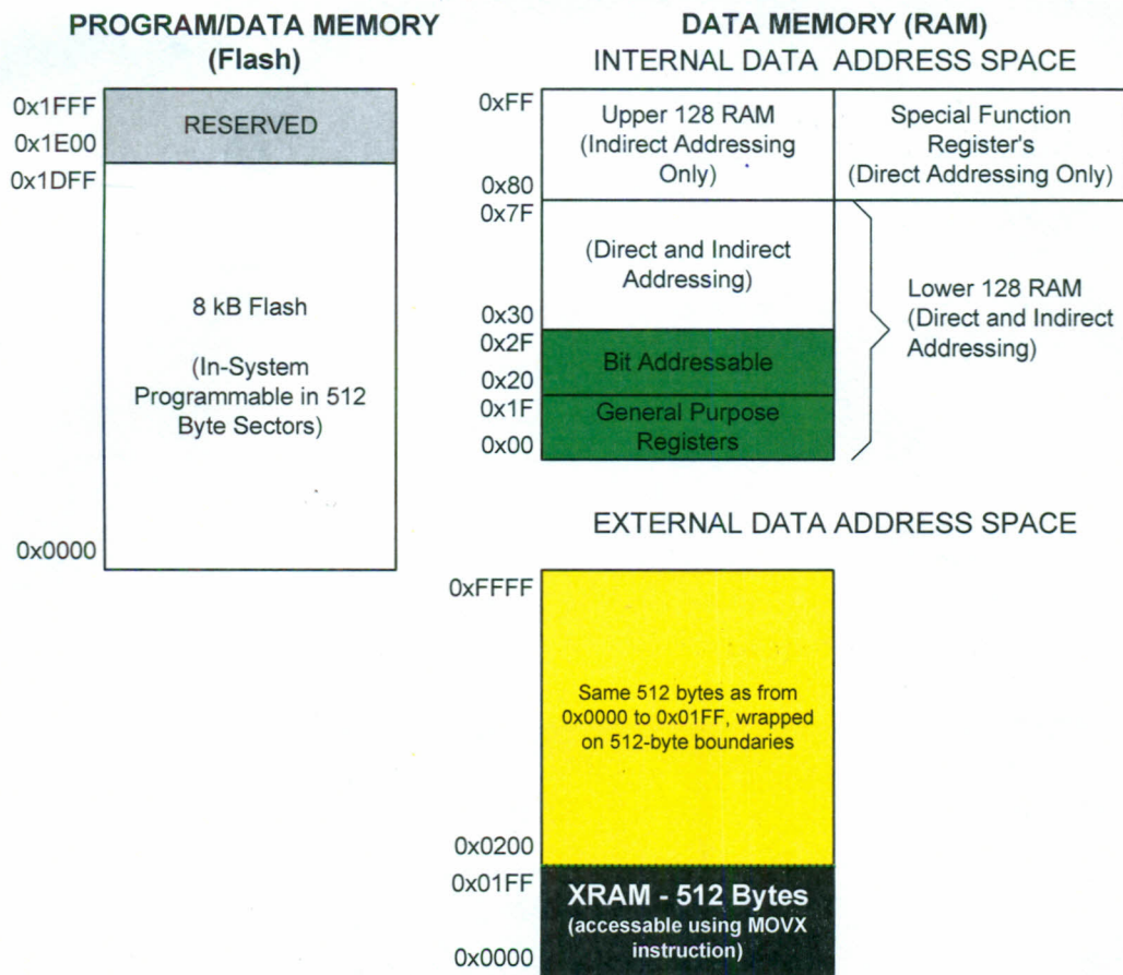
Figure 1.6. Memory Map
