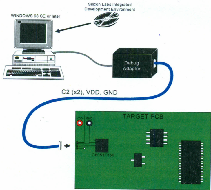
Figure 1.5. Development/In-System Debug Diagram
